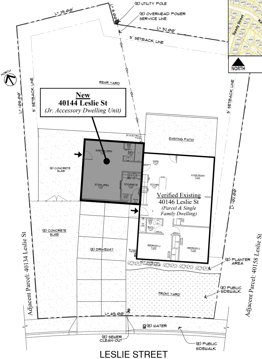
LOCATIONAL MAP
