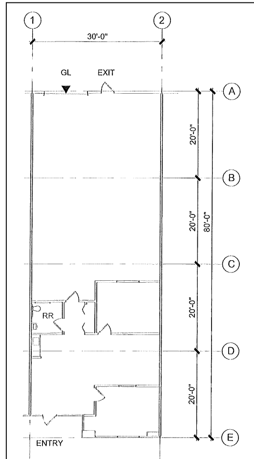
46707 Fremont Blvd (Floor plan of tenant space)
