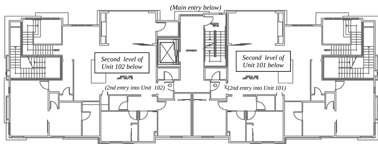
Second Floor
