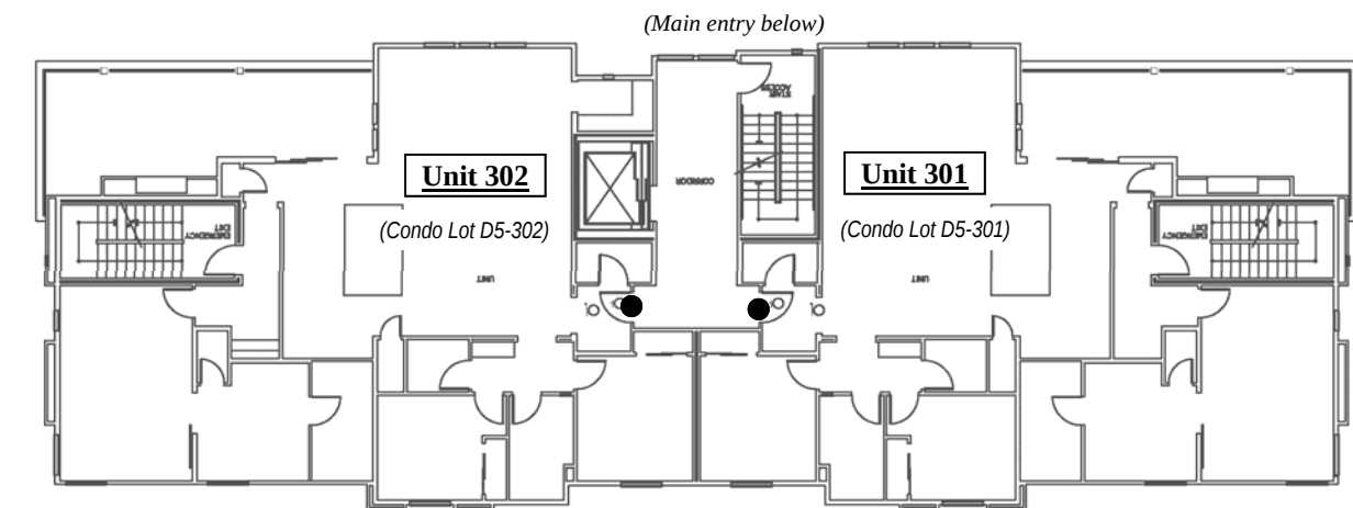
Third Floor
