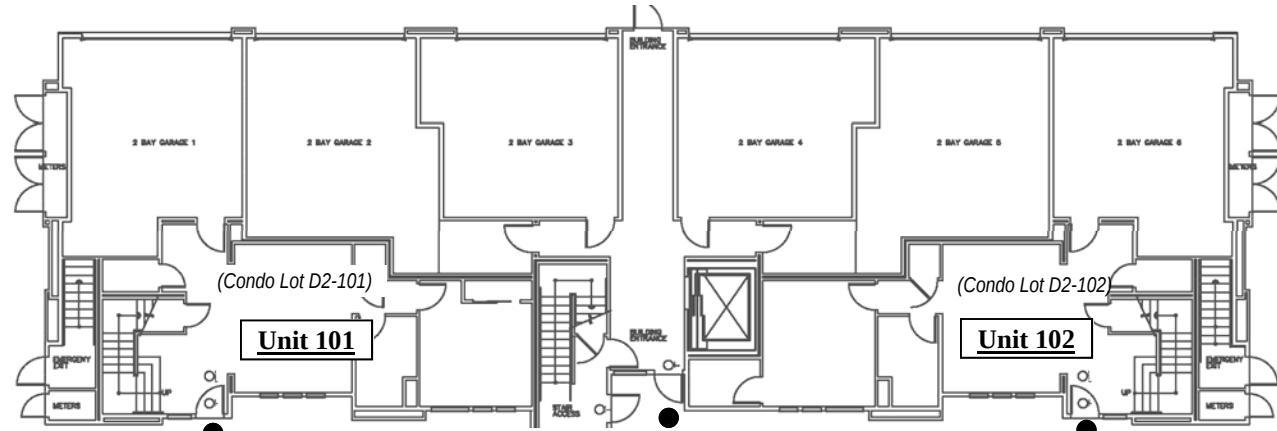
First Floor
