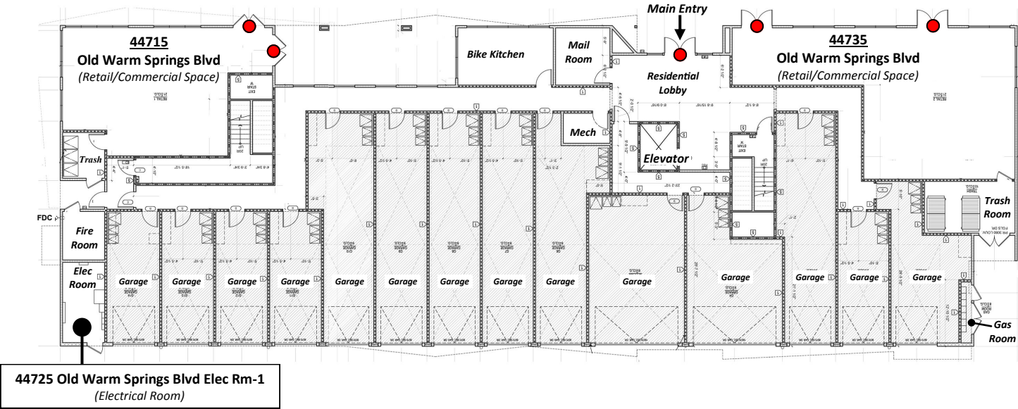
FIRST FLOOR (GROUND LEVEL)
